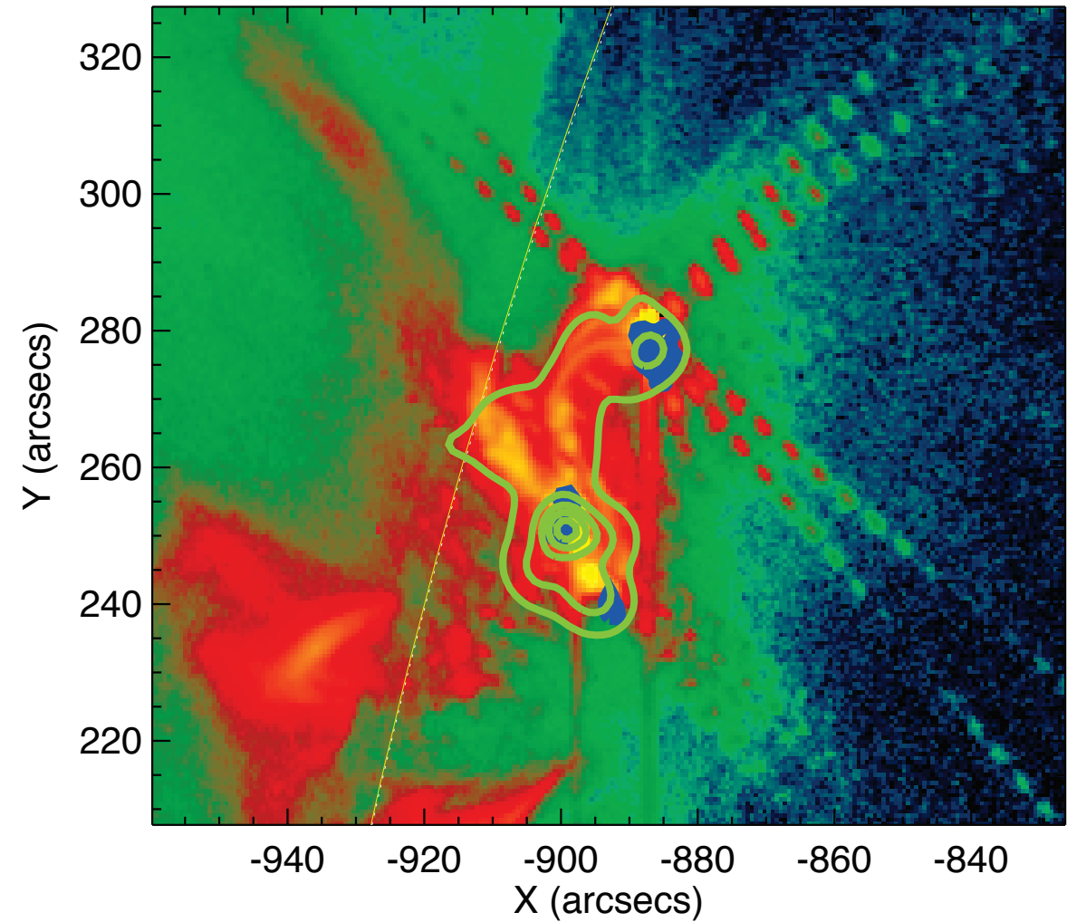
SDO AIA_4 94 5-May-2015 22:07:49.120 UT
