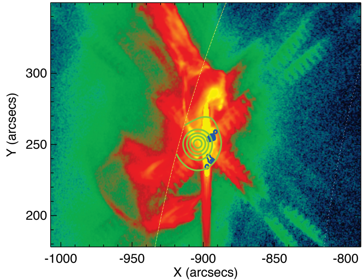
SDO AIA_4 94 5-May-2015 22:09:37.120 UT
