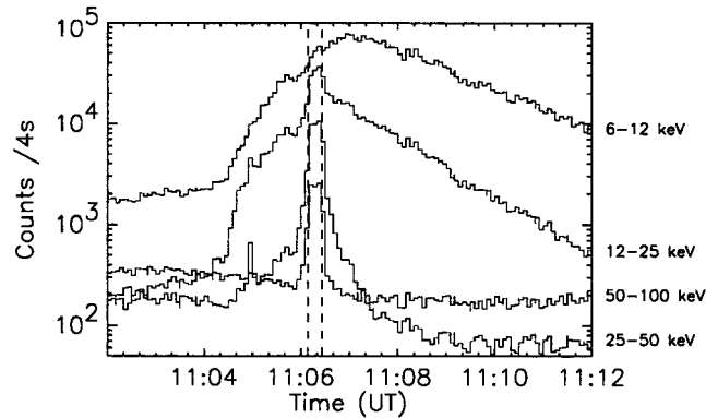
Figure 1. RHESSI light curves in four energy bands. The count rate (4-s time integration) is summed over detectors 1 through 9, excluding detectors 2 and 7. For clarity, we have scaled the count rates by 5.0 (6–12 keV), 1.5 (12–25 keV), 1.0 (25–50 keV), and 1.0 (50–100 keV). The two vertical lines show the integration time interval for the RHESSI images and spectra in this paper.
