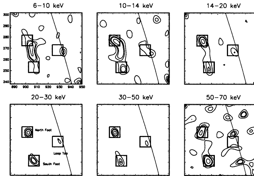
Figure 3. Images obtained with the MEM-Sato algorithm. The time interval is 11:06:10–11:06:24 UT. The contour levels are 0.08, 0.2, 0.3, 0.7. The contour levels are normalized to the peak flux of each image. The smooth line shows the location of the solar limb. The three boxes indicate the pixels that were summed to obtain the footpoint and loop-top spectra in Figure 5.
