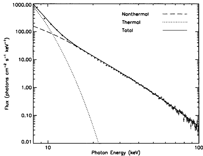
Figure 2. RHESSI spatially integrated, background-subtracted photon spectrum for the time interval 11:06:10–11:06:24 UT, the same as that for all RHESSI images shown later. The bremsstrahlung spectrum from an isothermal plasma plus a double power-law electron distribution (both shown separately on the plot, in addition to the total spectrum) were fit to the RHESSI count data to obtain this spectrum.
