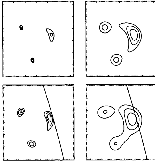
Figure 10. An unprocessed image from the flare model ( top left ), the same image convolved with a 7 arc sec FWHM conical response function ( top right ), the same image processed with MEM-Sato ( bottom left ), and the image processed with CLEAN ( bottom right ) are shown. Contour levels are 0.2, 0.4, and 0.7 times the peak flux in each image.
