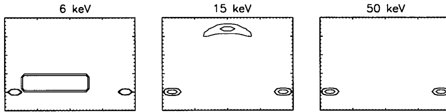
Figure 6. Model flare loop images at 6 keV, 15 keV, and 50 keV. Contour levels are 0.05, 0.07, and 0.5 times the peak flux in each image. The spatial resolution is 1 arc sec. These images are not rotated and scaled to the RHESSI images.
