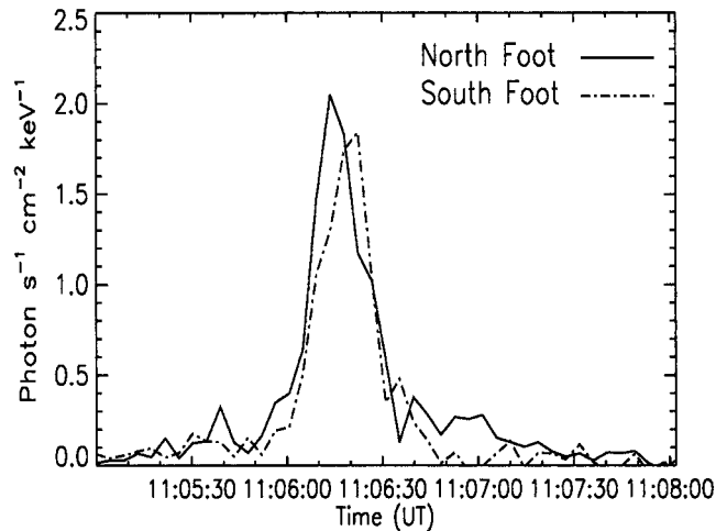
Figure 12. Emission history of the two footpoints at 20–25 keV. The start time is 11:05:00 UT. The peak of the north footpoint emission is earlier than the peak of the south footpoint emission by about 8 seconds.
