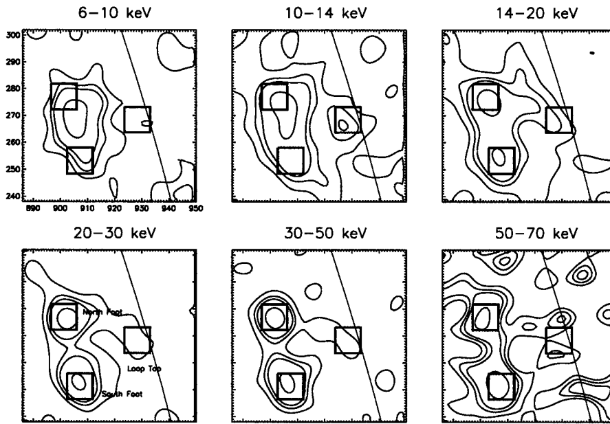
Figure 4. Images obtained with the CLEAN algorithm. All other aspects are the same as in Figure 3.
