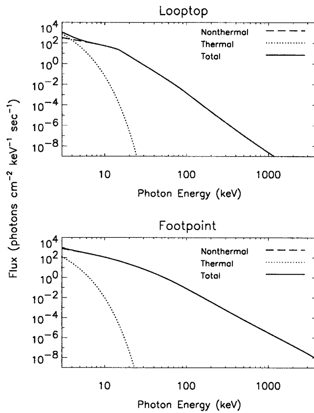
Figure 7. Spectra from the model loop images. The top panel shows the spectrum from the loop top and the bottom panel shows the spectrum from a footpoint. The dashed curve is the total non-thermal bremsstrahlung from a footpoint or the loop top, the dotted curve is the thermal bremsstrahlung from the same region, and the solid curve is the total spectrum.
