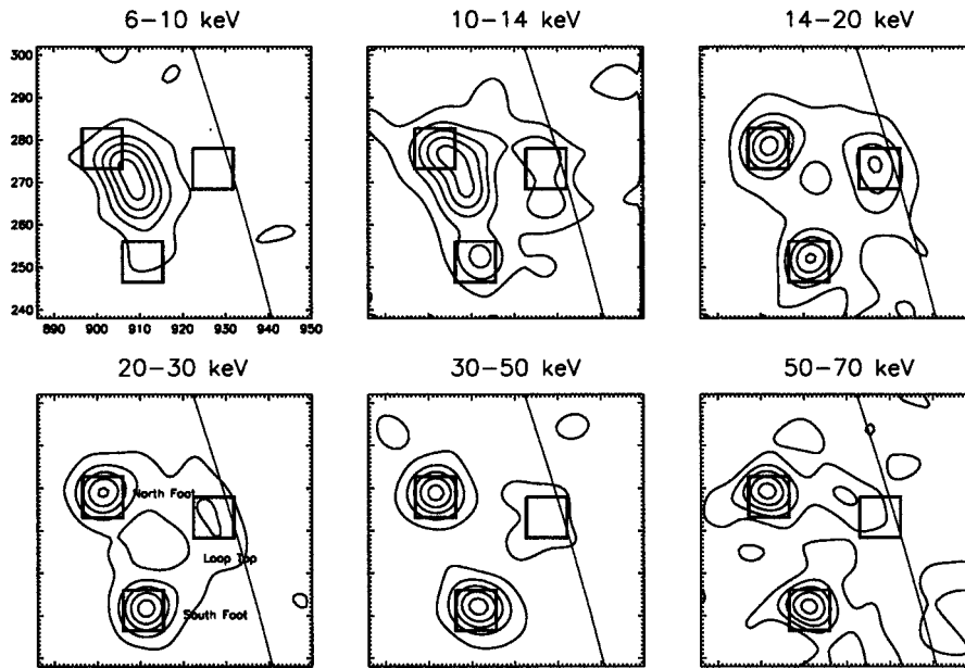
Figure 9. CLEAN images of the model flare loop. Contour levels are the same as Figure 8.
