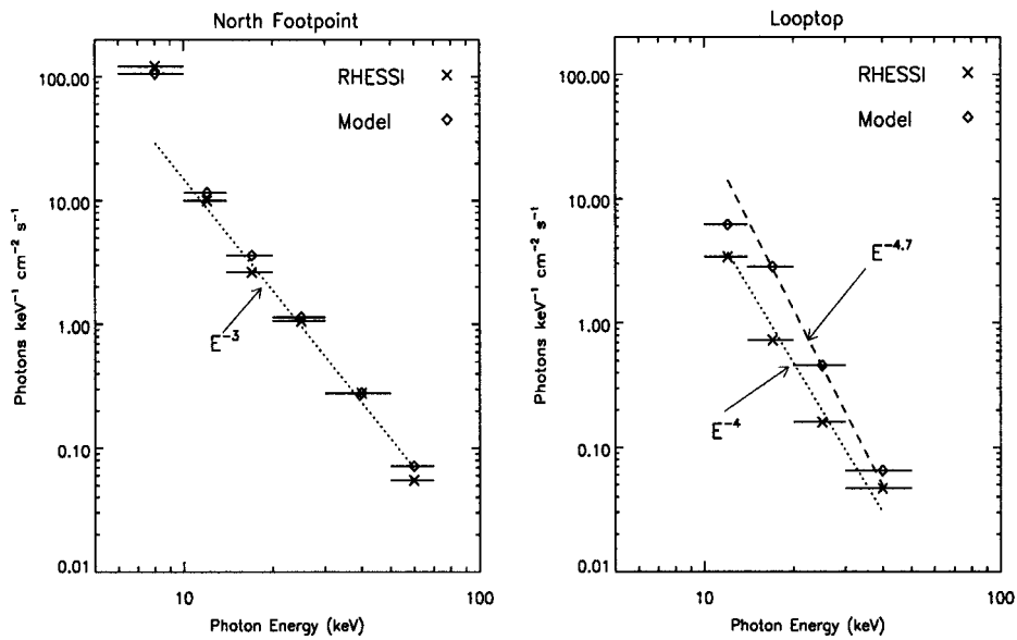
Figure 5. Spectra for the north footpoint ( left panel ) and loop top ( right panel ). The horizontal bars marked with an ‘x’ are from the CLEAN images shown in Figure 4. The bars marked with a diamond are from the model images reconstructed with CLEAN (Figure 9). The time interval is the same as that for Figures 3 and 4.
