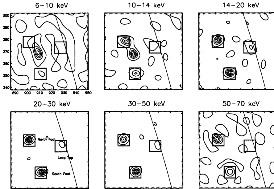
Figure 8. MEM-Sato images of the model flare loop. Contour levels are 0.1, 0.3, 0.5, 0.7, and 0.9. The contours are normalized to the peak flux of each image. As in Figures 3 and 4, the smooth line is the solar limb.
