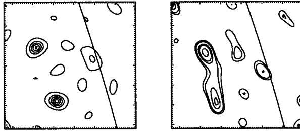
Figure 11. MEM-Sato 14–20 keV images of the model ( left ) and of the observed flare ( right ). We can see similar patterns in them. The sources between the loop top and footpoints in the left image are not real. Consequently, we deduce that sources between the footpoints and the loop top in the right image are also not real.
