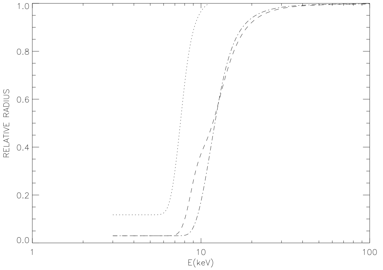
HESSI EFFECTIVE SHUTTER RADIUS - subcoll 3
