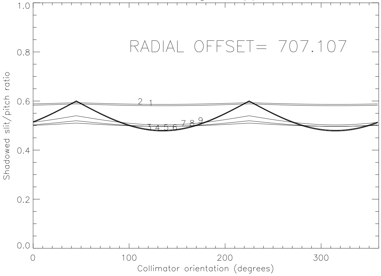
Effect of shadowing on slit/pitch ratios
